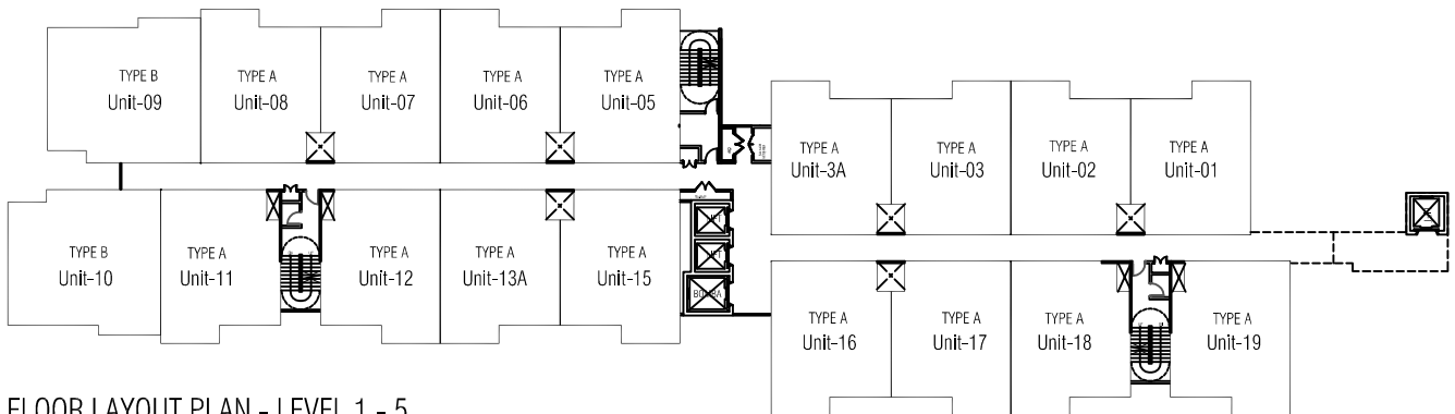
FLOOR LAYOUT PLAN - LEVEL 1 - 5
